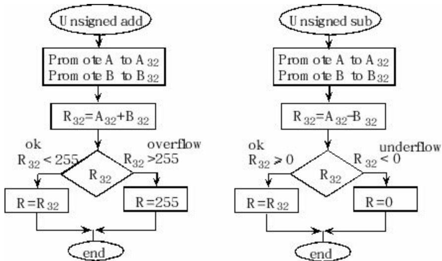
Figure 3.23. Flowcharts showing how to use promotion to detect and correct unsigned arithmetic errors.
