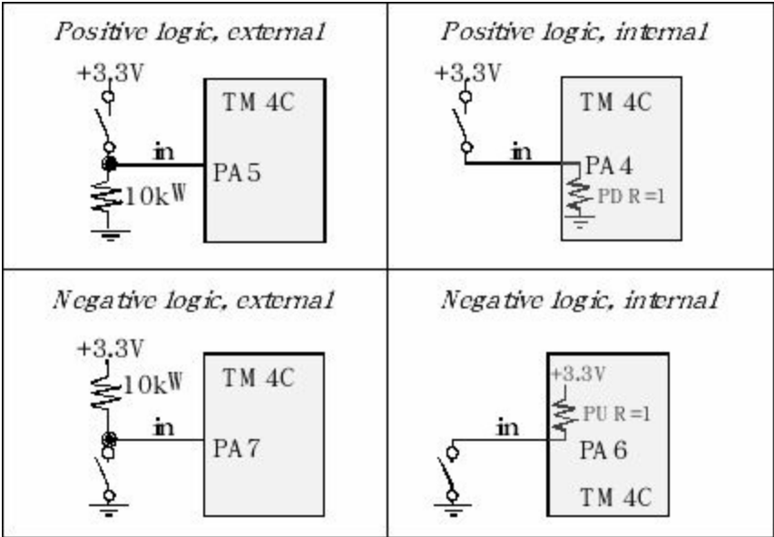
Figure 4.15. Interface of a switch to a microcomputer input.
