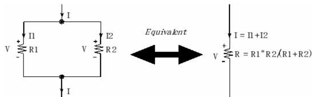
Figure 1.7. The parallel combination of two resistors, R_1 R_2 , is equivalent to one resistor at R_1 * R_2 / (R_1 + R_2) .
