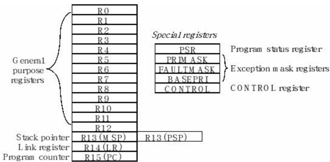
Figure 3.2. Registers on the ARM® Cortex-M processor.
