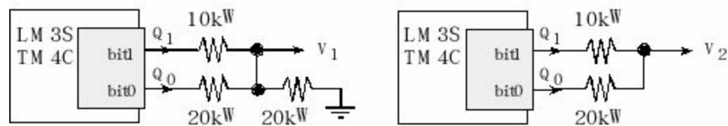
Figure 10.4. Two solutions for a 2-bit binary-weighted DAC.
