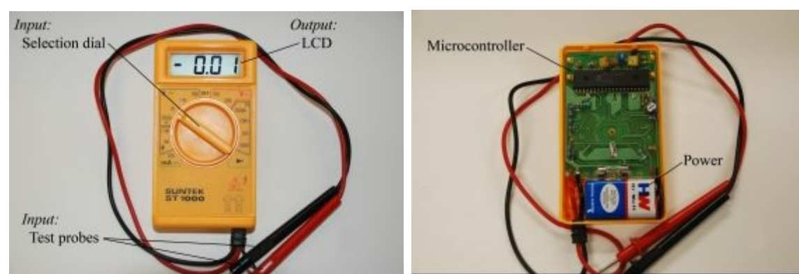
Figure 2.2. A digital multimeter contains a microcontroller programmed to measure voltage, current and resistance.
