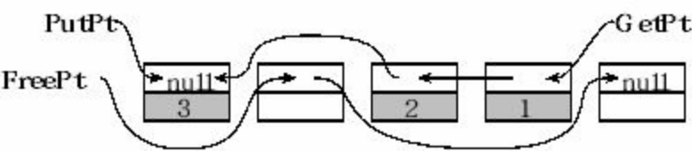
Figure 6.12. A linked list FIFO after putting 1,2,3.
