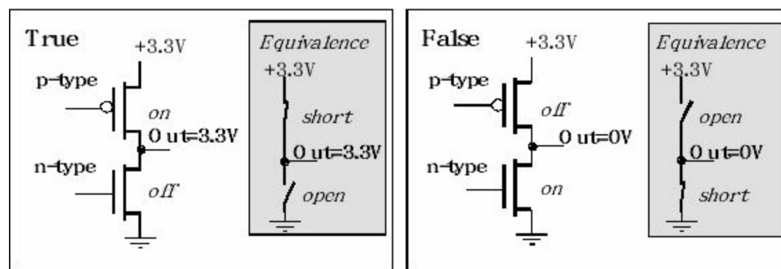
Figure 1.8. A binary bit at the output is true if a voltage is present and false if the voltage is 0.
