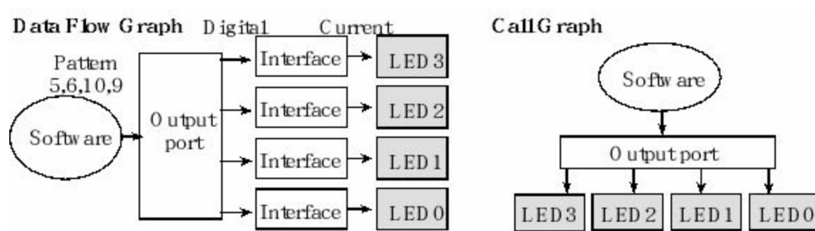
Figure 4.19. Data flow graph and call graph of the LED output system.
