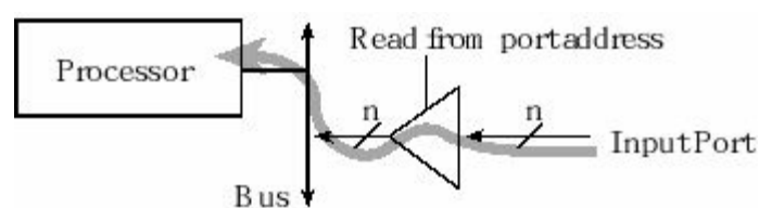
Figure 4.11. A read only input port allows the software to sense external digital signals.
