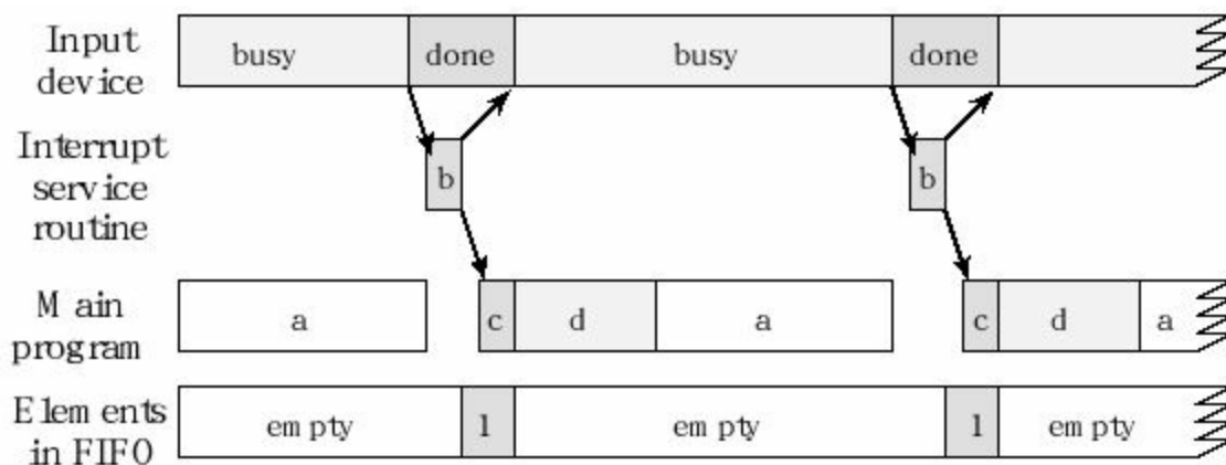
Figure 11.8. Hardware/software timing of an I/O bound input interface.
