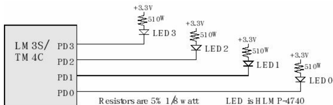
Figure 4.20. Hardware circuit for the LED output system.
