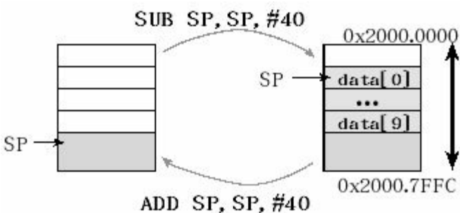
Figure 7.2. A stack picture showing a local array of ten elements.
