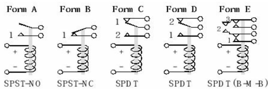
Figure 8.18. Standard relay configurations.
