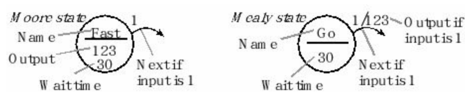
Figure 6.7. The output in a Moore depends just on the state. In a Mealy the output depends on state and input.
