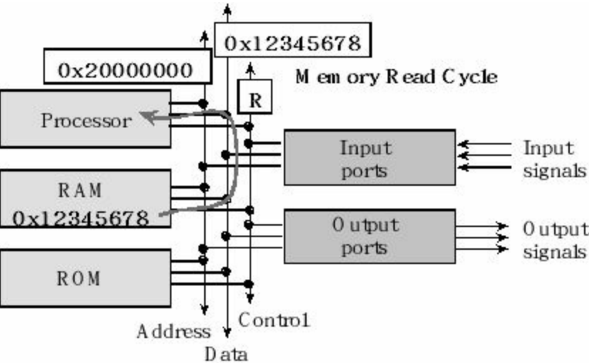
Figure 3.31. A read cycle copies data from RAM, ROM or input device into the
