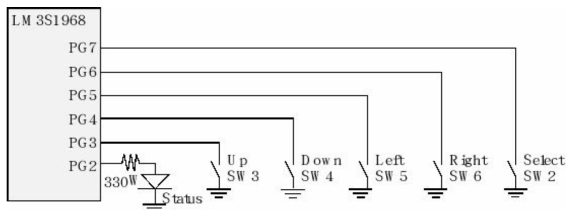
Figure 4.2. Evaluation kit for the LM3S1968 microcontroller.
