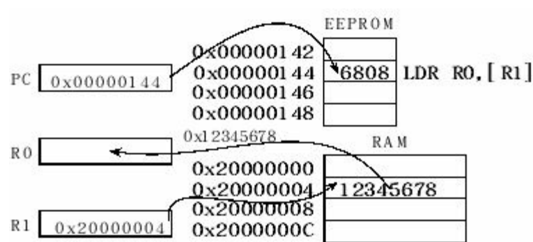
Figure 3.11. An example of indexed addressing mode, data is in memory.
