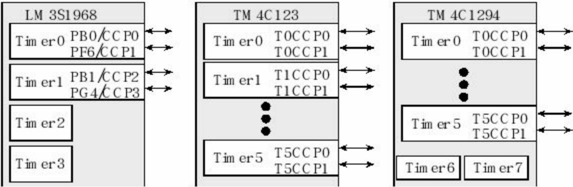
Figure 9.13. Timer pins on the LM3S/TM4C microcontroller are labeled CCP.
