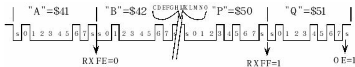
Figure 8.7. Seventeen receive data frames result in an overrun (OE) error.
