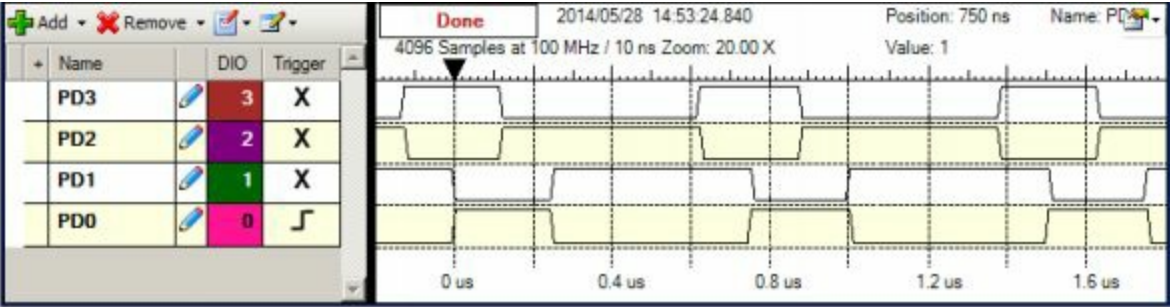
Figure 4.22. Logic analyzer waveforms collected during the testing of the LED output system.
