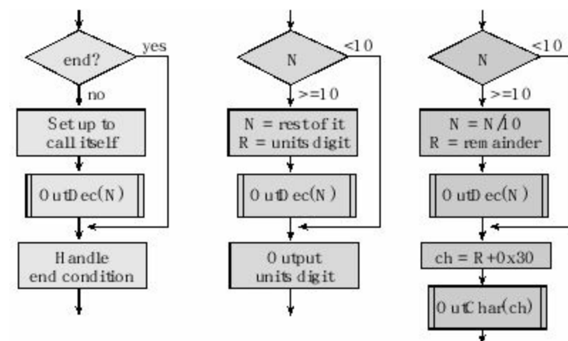
Figure 5.12. Successive refinement method for the recursive approach.
