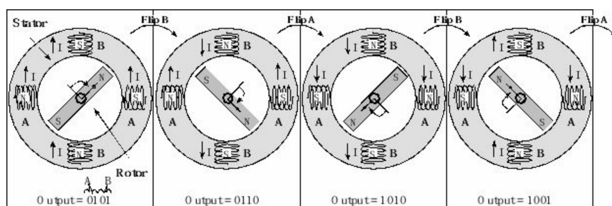
Figure 8.23. To rotate this stepper by 18^\circ , the interface flips the direction of one of the currents.
