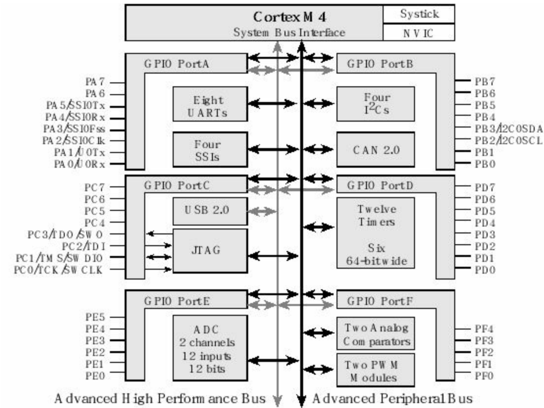
Figure 4.4. I/O port pins for the LM4F120H5QR / TM4C123GH6PM microcontrollers.
