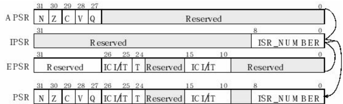
Figure 3.3. The program status register of the ARM® Cortex-M processor.
