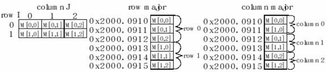
Figure 6.14. A byte matrix with 2 rows and 3 columns.
