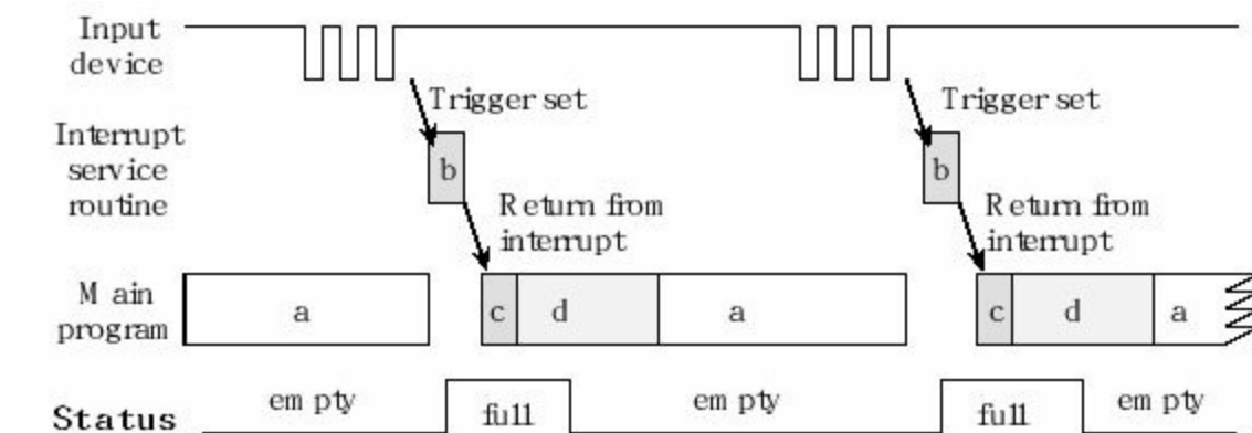
Figure 9.7. Hardware/software timing of an input interface using a mailbox.
