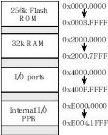
TM4C123
