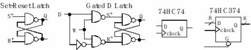
Figure 1.14. Digital storage elements.
