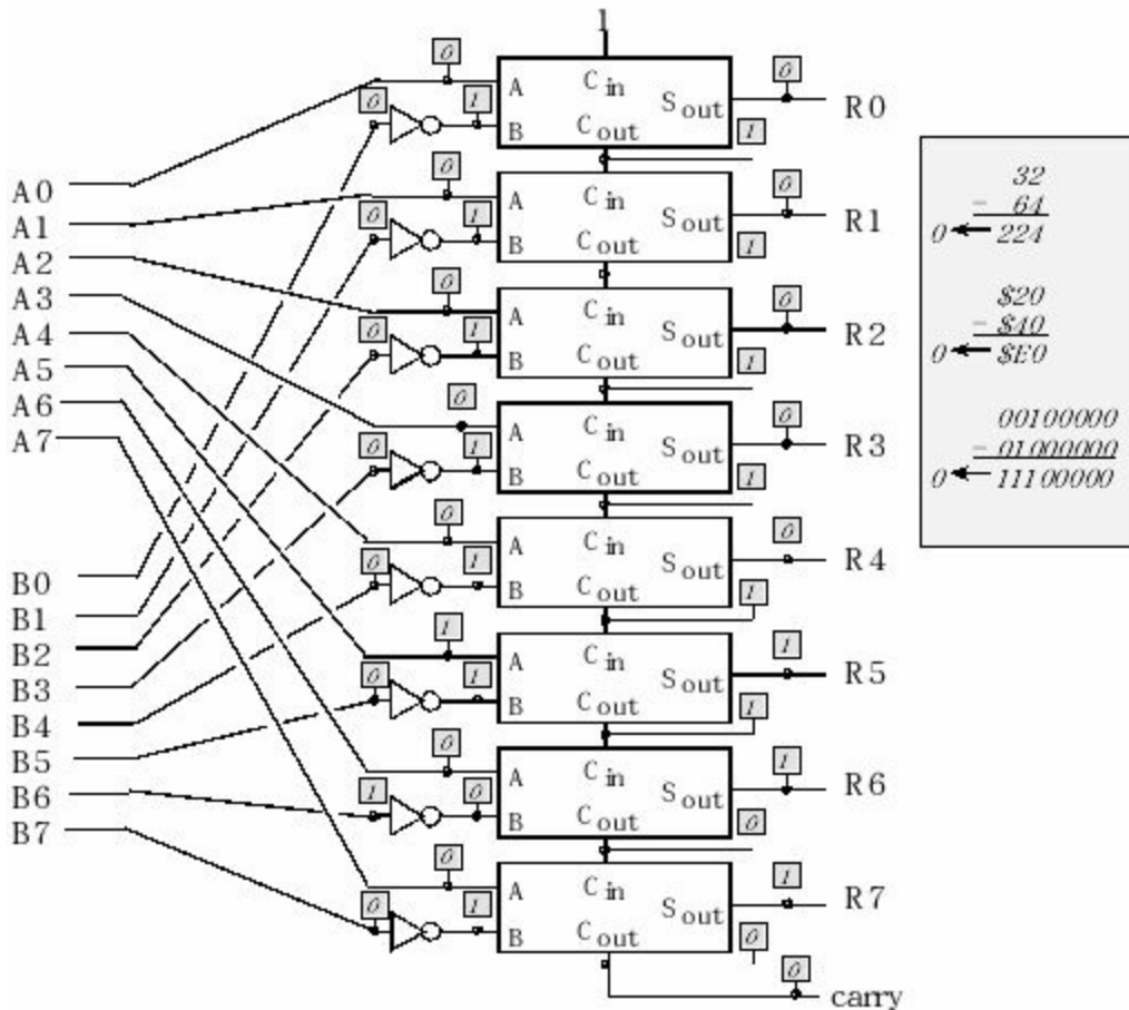
Figure 3.19. We make an 8-bit subtractor using eight binary full adders. Carry out is 0 in this case because the unsigned result is incorrect.
