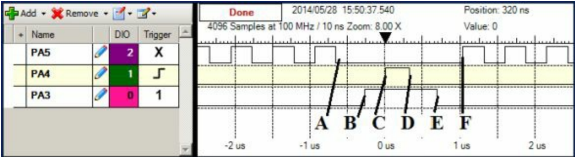
Figure 9.15. Real-time thread profile measured with a logic analyzer. Trigger is set for condition PA3 is high (running Timer0 ISR) and rising edge of PA4 (start of SysTick ISR).
