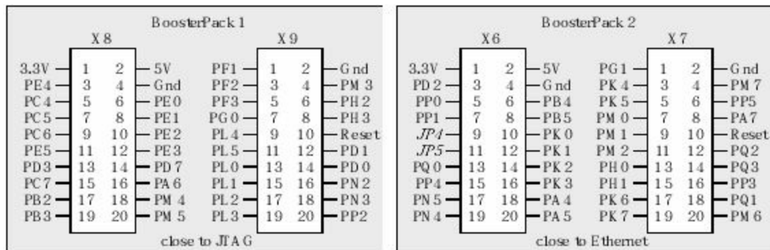
Figure 4.8. Interface connectors on the EK-TM4C1294-XL LaunchPad Evaluation Board.
