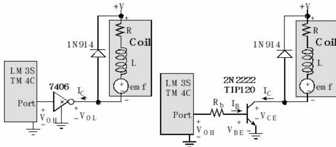
Figure 8.16. Binary interface to EM relay, solenoid, DC motor, or speaker.
