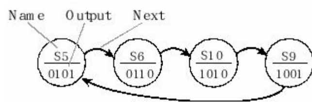
Figure 8.24. This stepper motor FSM has four states. The 4-bit outputs are given in binary.
