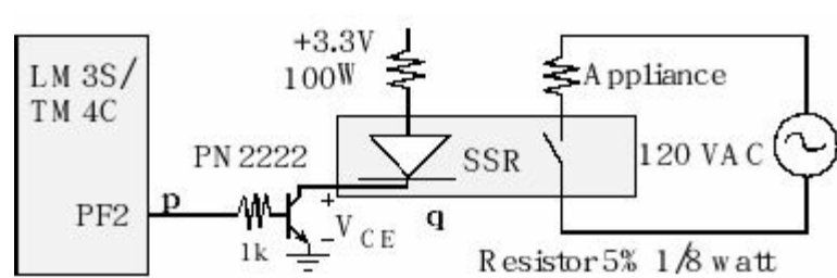
Figure 4.18. Solid state relay interface using a PN2222 NPN transistor.
