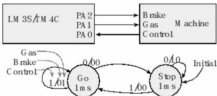
Figure 6.10. Engine controller implemented with a Mealy FSM.
