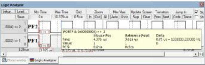
Figure 4.17. Logic analyzer in the Keil uVision simulator measures the frequency of the squarewaves.
