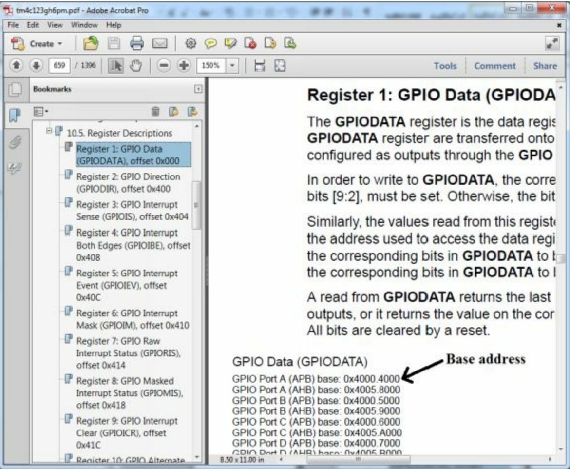
Figure 4.14. Snapshot of the TM4C123 data sheet, showing how to look up GPIO base addresses.
