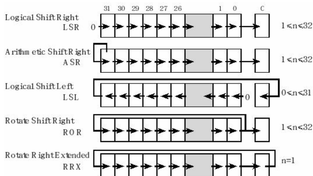
Figure 3.14. Shift operations.
