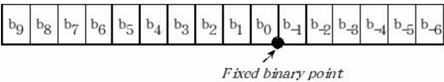
Figure 1.24. 16-bit binary fixed-point format with \Delta = 2^{-6} .
