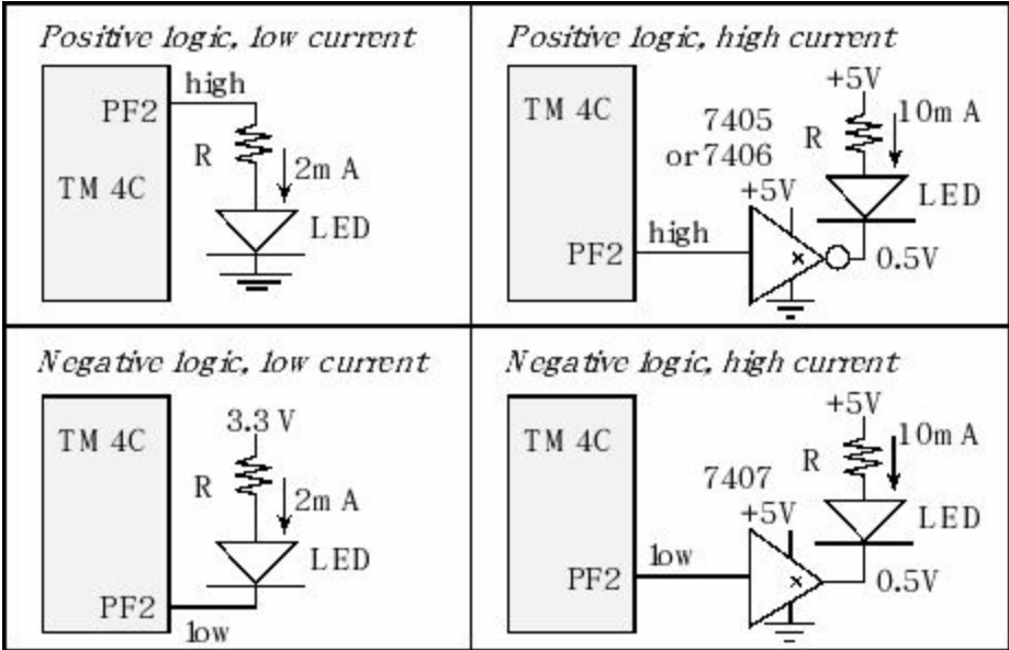
Figure 4.16. Four LED interface circuits to a microcontroller output.
