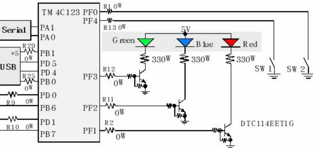
TM4C123 LaunchPad (LM4F120 is the same except no R25 and R29)
