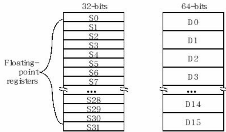
Figure 7.12. The TM4C has 32 single-precision floating-point registers that overlap with 16 double-precision floating-point registers.
