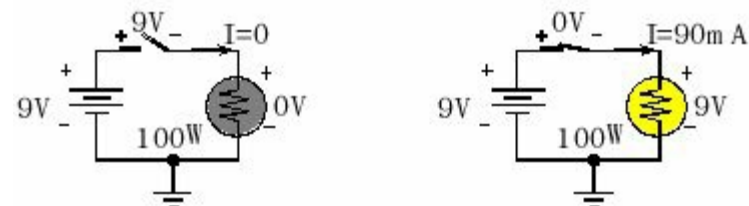
Figure 1.4. The voltages around a loop will sum to zero (KVL).
