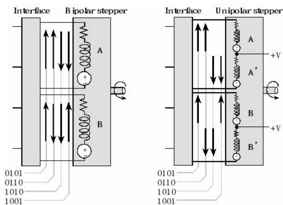
Figure 8.22. A bipolar stepper has 2 coils, but a unipolar stepper divides those two coils into four parts.
