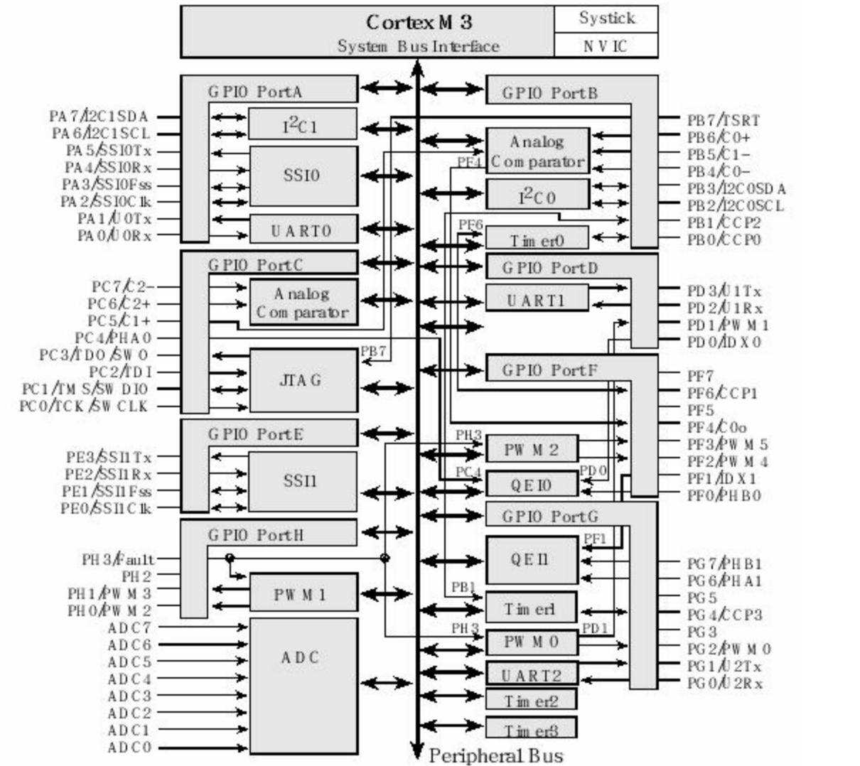
Figure 4.1. I/O port pins for the LM3S1968 microcontroller.
